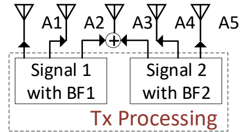
Fig. 10: Two virtual subarrays with one overlapped antenna are formed: Virtual subarray 1 with antennas A1, A2 and A3; and subarray 2 with A3, A4 and A5. Each virtual subarray will transmit one data signal, and the signals between two virtual subarrays are orthogonal over time. Beamforming is applied in each virtual subarray. BF for beamforming.
