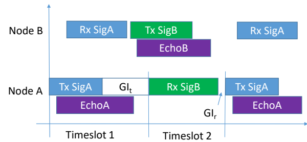
Fig. 7: Illustration of the timeslot allocation in a full-duplex TDD JCAS system from the viewpoint of Node A. Full-duplex operation is only required during timeslot 1. GI stands for guarding interval, “Sig” is a shortened form of signal.
