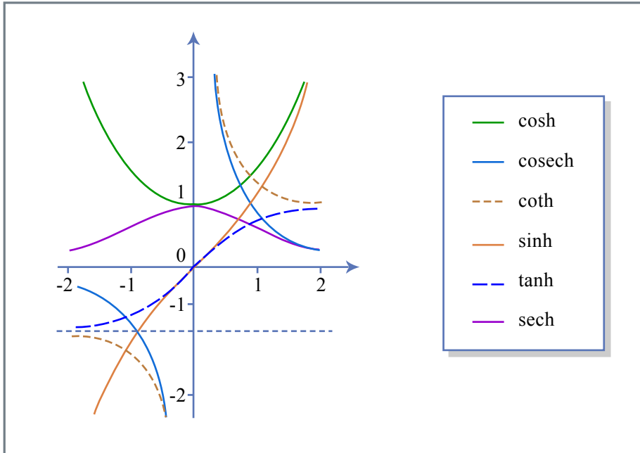
Figure 3.26: Hyperbolic functions
