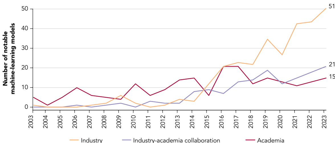
Number of notable machine-learning models by sector, 2003–23
