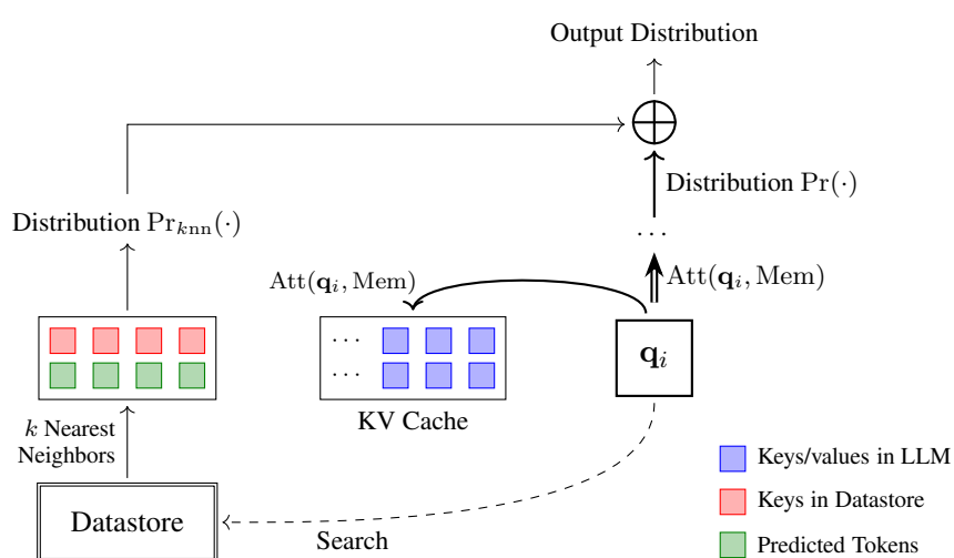
(b) k -NN Language Modeling
