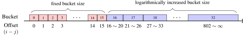
Fig. 2.10: Illustration of distributing query-key offsets into buckets in the T5 model ( n_b = 32 and \text{dist}_{\max} = 1024 ). Boxes represent buckets. In the first half of the buckets, we use a fixed bucket size. In the second half of the buckets, we increase the bucket size logarithmically. The last bucket contains all the query-key offsets that are not covered by previous buckets.
