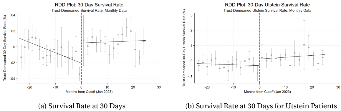
Figure 8: Regression Discontinuity in Time: Survival Rate at 30 Days
