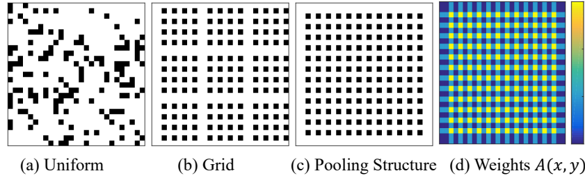
Fig. 3. Input-independent perforation masks in PerforatedCNNs . According to the paper, the mass layout is for the AlexNet Conv2 layer. (a) Uniform perforation mask is N points chosen randomly without replacement from the set \Omega . (b) Grid perforation mask is a set of points I = a(1), \dots, a(Kx) \times b(1), \dots, b(Ky) the values of a(i) , b(i) using the pseudorandom integer sequence generation scheme [59]. (c) Pooling structure mask exploits the structure of the overlaps of pooling operators. Denote by A(x, y) the number of times the convolutional layer output is used in the pooling operators. The pooling structure mask is obtained by picking top- N positions with the highest values of A(x, y) . (d) Impact mask estimates the impact of perforation of each position on the CNN loss function and then removes the least important positions. When activation maps are computed, the coordinates of black pixels are skipped. Figures and description adapted from reference [49].
