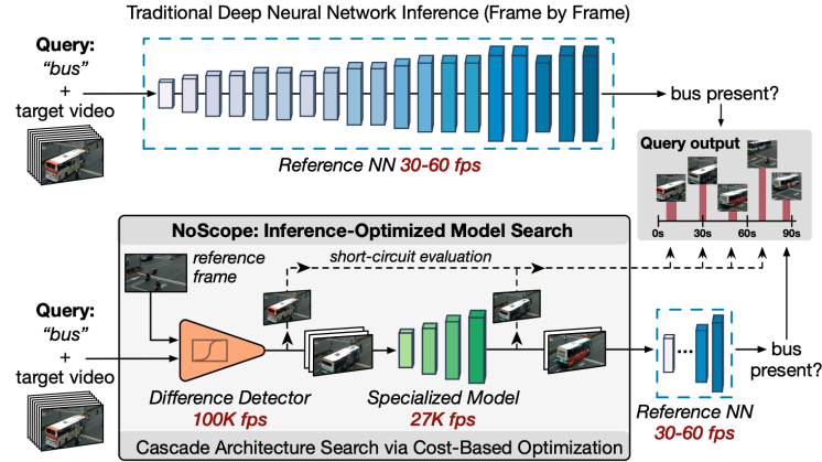
Fig. 7. Illustration of the NoScope framework. NoScope is a system for accelerating neural network analysis over videos via an inference-optimized model search. Given an input video, target object, and reference neural network, NoScope automatically searches for and trains a cascade of models—including difference detectors and specialized networks—that can reproduce the binarized outputs of the reference network with high accuracy—but up to three orders of magnitude faster. Figure and description adapted from reference [84].
