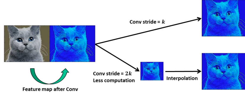
Fig. 6. Illustration of virtual polling [104]. By using a larger stride, it save computation in conv layers and, to recover the output size, it use linear interpolation which is fast to compute. Figure and description adapted from reference [27].
