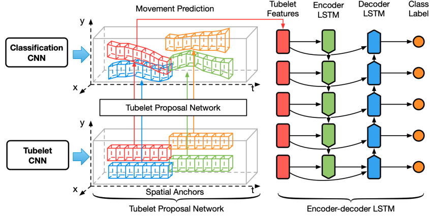
Fig. 16. The proposed object detection system consists of two main parts. The first is a tubelet proposal network to generate tubelet proposals efficiently. The tubelet proposal network extracts multi-frame features within the spatial anchors, predicts the object motion patterns relative to the spatial anchors, and generates tubelet proposals. The gray box indicates the video clip, and different colors indicate the proposal process of other spatial anchors. The second part is an encoder-decoder CNN-LSTM network to extract tubelet features and classify each proposal box into different classes. The tubelet features are first fed into the encoder LSTM by a forward pass to capture the appearance features of the entire sequence. Then the states are copied to the decoder LSTM for a backward pass with the tubelet features. The encoder-decoder LSTM processes the whole clip before outputting class probabilities for each frame. Figure and description reference adapted from reference [86].
