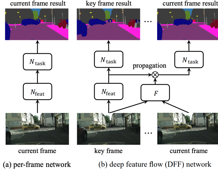
Fig. 13. Illustration of temporal propagation in deep feature flow . (a) Video recognition using per-frame network evaluation (b) The proposed deep feature flow . Figures and descriptions adapted from reference [169].
