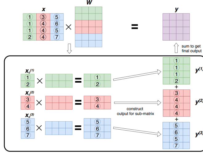
Fig. 2. Illustration of sub-vector clustering in Deep Reuse . In a convolution layer, the activation maps of 2D images are unfolded as x and are multiplied by weights W of corresponding filters. With sub-vector clustering, x is first divided into sub-vectors and labeled with corresponding cluster ids. In the matrix multiplication, only the representative of each cluster is used. Afterward, the output activation maps are re-constructed with the representative results of each cluster. Figure adapted from reference [116].
