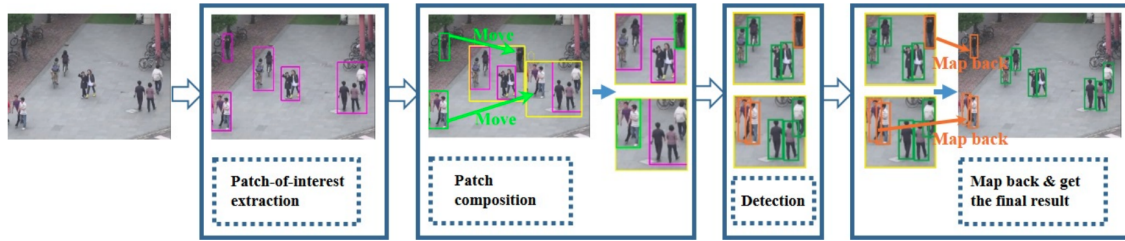
Fig. 10. Patch-of-Interest composition. (a) The input image. (b) Detected patches. (c) The patch composition (left) and sub-frames(right). (d) Detection results on sub-frames. (e) Map back and get the final result on the original image. Figures and descriptions adapted from reference [162].
